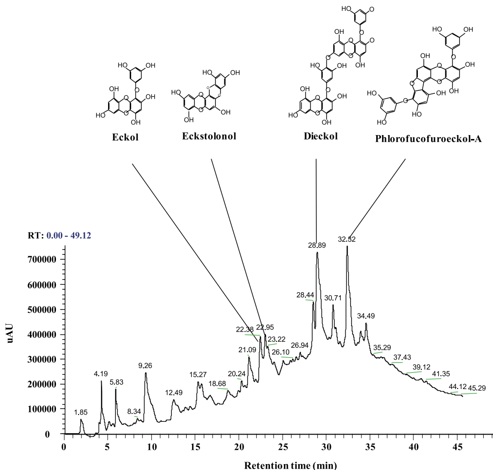
Fig. 1. High-performance liquid chromatography (HPLC) chromatogram and HPLC-diode array detection / electrospray ionization mass spectrometry spectra of ethyl acetate fraction from Ecklonia cava processing by-product.
